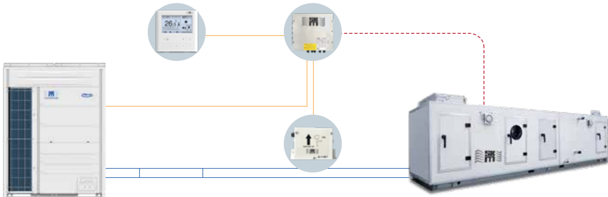
VRF + AHU CONNECTION SOLUTION
